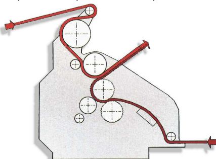
Corrugated board machine from FARO International GmbH
